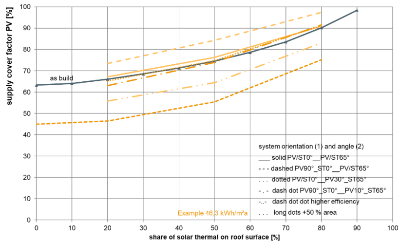
Figure 11: Supply cover factor for PV system
